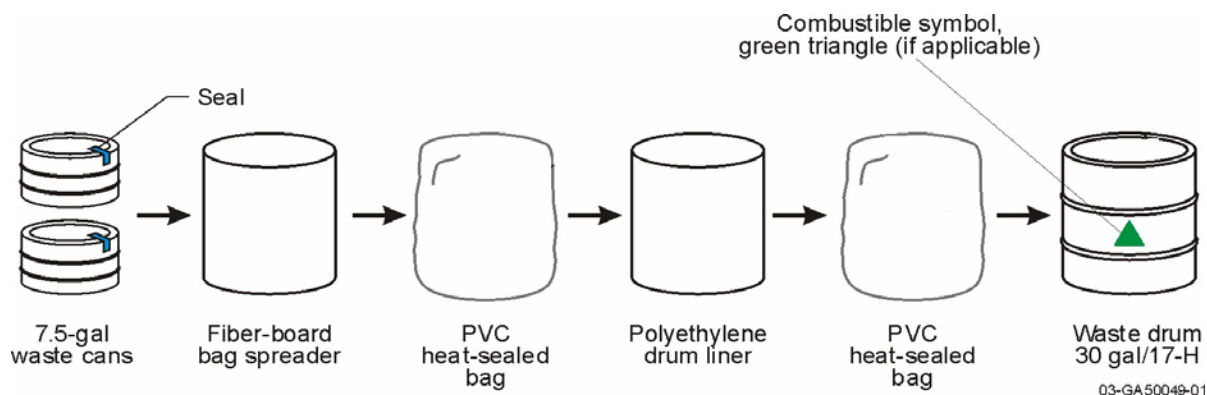
Fig. 1. Schematic of 30-gallon (114-L) drum packaging.
