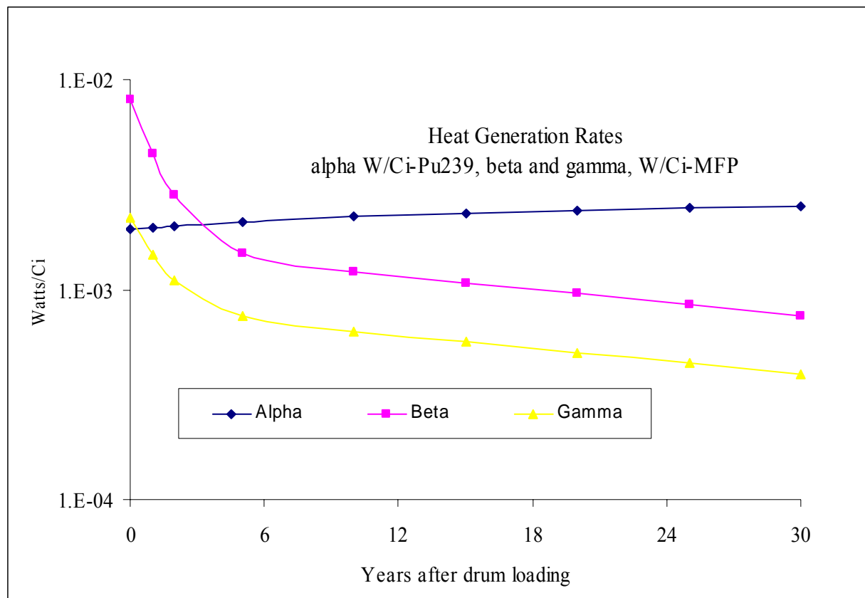
Fig. 2. Decay heat generation rates in a typical RH-TRU waste drum stored at INEEL.
