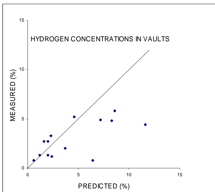
Fig. 3. Comparison of the code-predicted and measured values of hydrogen concentration.
