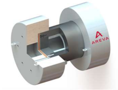
Fig. 2. TN ® MW cask with shock absorbers for transportation configuration
