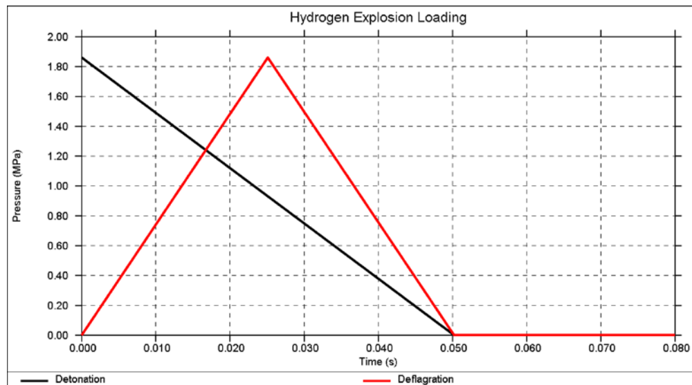
Figure 2 - Hydrogen Explosion Loading
