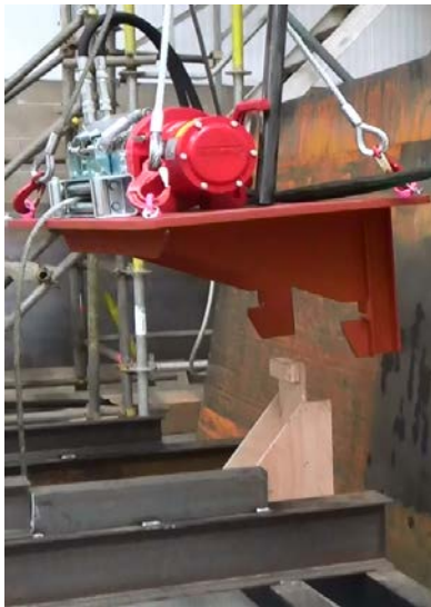
Fig. 17. Hydraulic Winch Deployment
