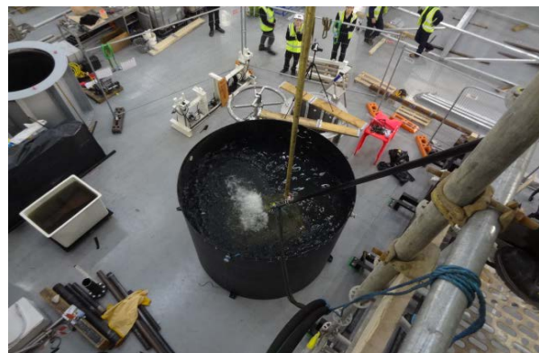
Fig. 10. Underwater Cutting Disc Trials
