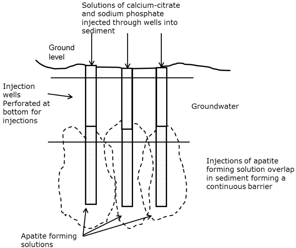
Figure 3. View of apatite deployed through injections wells into groundwater to form an apatite permeable reactive barrier and provide source area treatment to the contaminated sediments.
