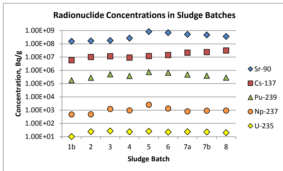
Figure 1. Concentrations of Select Radionuclides in SRS Sludge Batches 1B through 8
