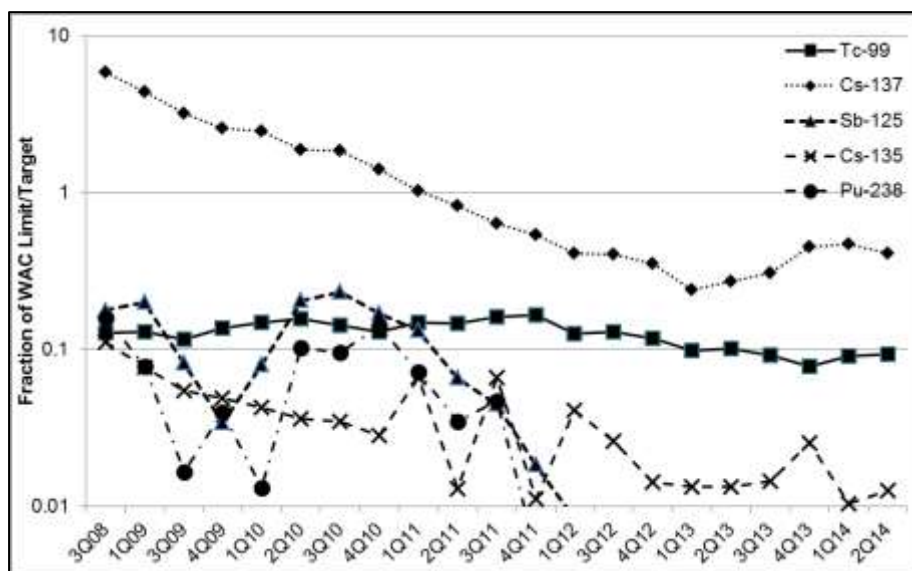
Figure 4. Radionuclides Exceeding 10% of the 2014 Saltstone WAC Limits/Targets
