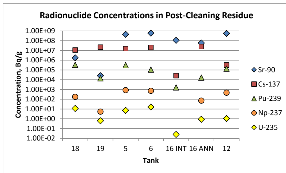
Figure 3. Concentrations of Select Radionuclides in SRS Post-Cleaning Residue
