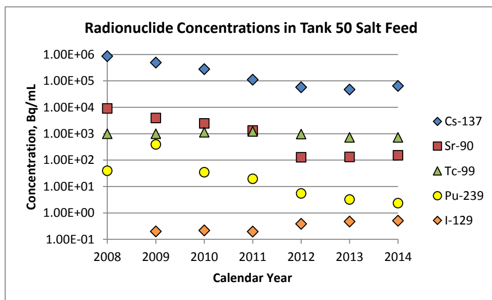
Figure 2. Concentrations of Select Radionuclides in SRS Tank 50 Salt Feed
