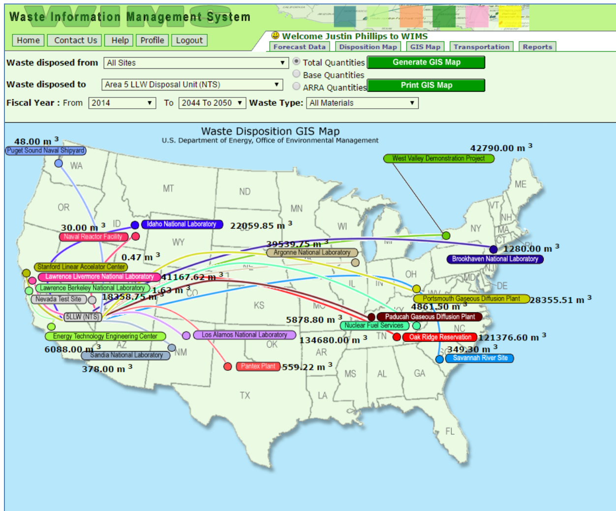
Fig. 3. The GIS map screen shot is displaying the waste forecasted to be sent from all DOE sites to the Area 5 LLW Nevada Test Site between the years 2014 and 2050.
