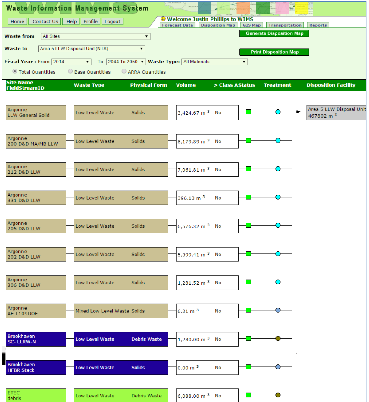
Fig. 2. The disposition map screen shot is displaying a sample of all the waste forecasted to be shipped to Area 5 LLW Nevada Test Site for disposition between the years 2014 and 2050.
