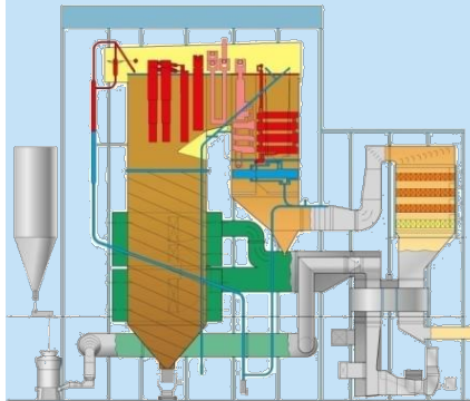
Ultra-Supercritical Boiler
