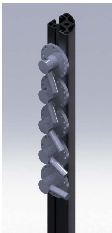
Figure 2: Design of the acoustic backscatter array (ABA).
