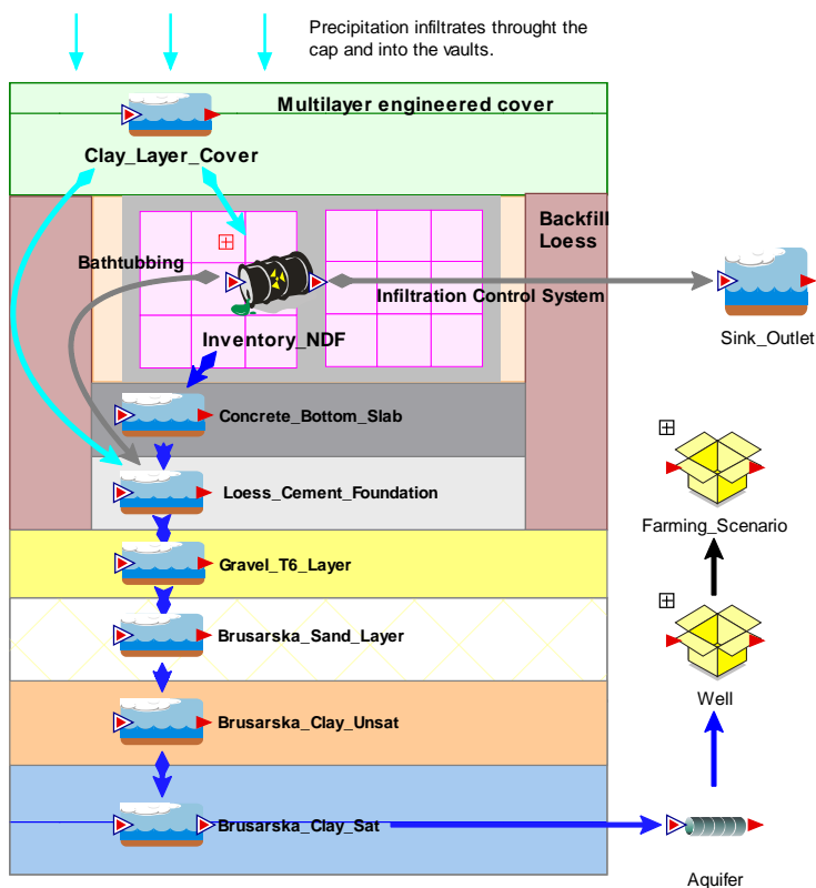
Fig. 3: Simplified GoldSim model for NDF Radiana.
