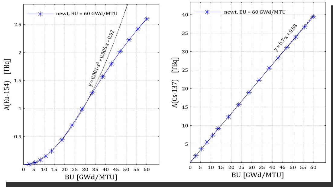
Fig. 7. Build-up of Eu-154 (left frame) and Cs-137 (right frame) as a function of burn up. Calculations are performed with SCALE 6.1 using newt model for burn ups < 60 GWd/MTU
