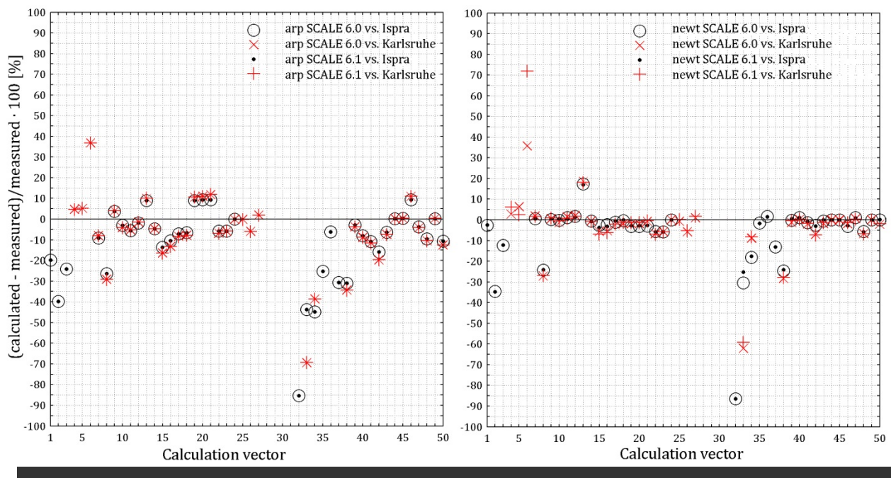
Fig. 4. Deviation between measured and simulated (left frame for arp model and right frame for newt model) data for the fuel element (BE 124) of the NPP Obrigheim. Measurement position RodG7p3, BU = 31.5 GWd/MTU
