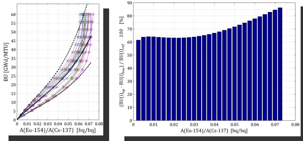
Fig. 8. Burn up as a function of the ratio Eu-154/Cs-137 (left frame) and the corresponding bandwidth (right frame). Calculations are performed with SCALE 6.1 using newt model for burn ups up to 60 GWd/MTU
