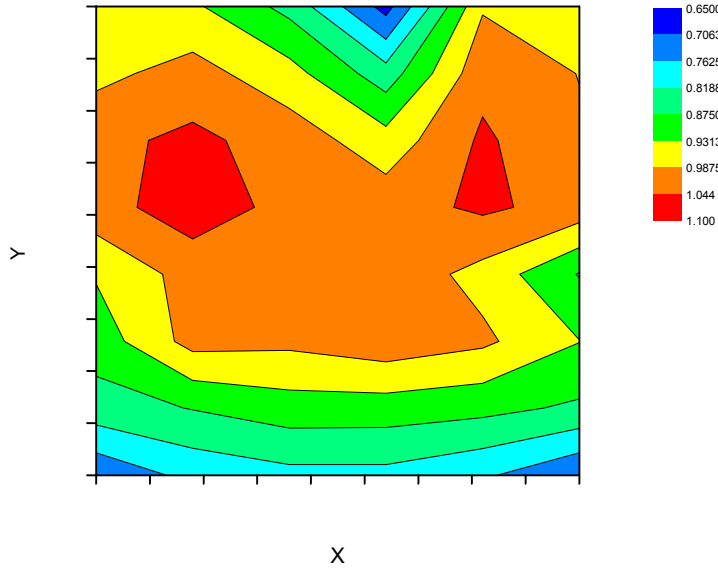
Figure 6. Contour plot of normalised experimental count rates. The values are normalised to the count rate of the central position on the tray, which is equal to 7.8 \text{ s}^{-1} . The two small highest count rate regions are believed to be an artifact of the choice of boundary values and relatively large counting errors.
