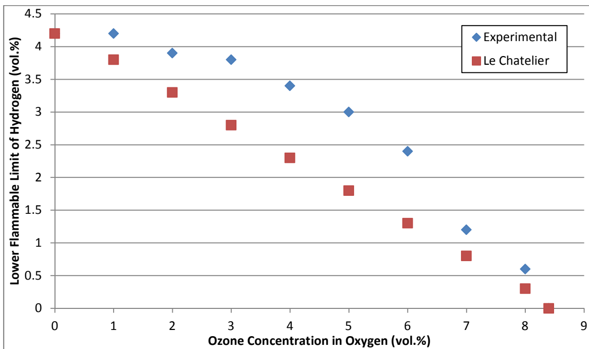
Figure 4: Lower flammable limit of hydrogen as a function of the ozone concentration
