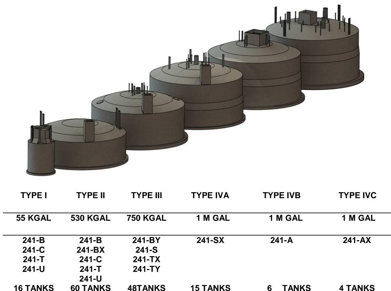
Figure 2 - Types, Sizes and Nominal Volumes of SSTs
