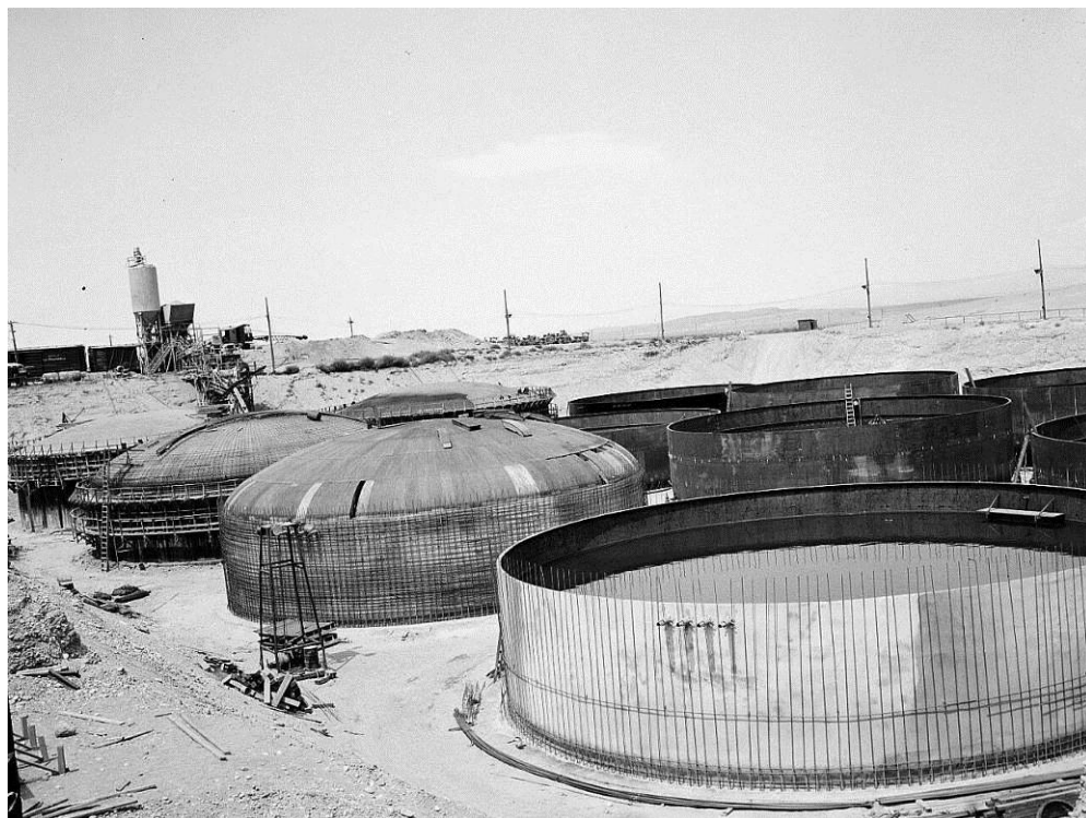
Figure 1 – BX tank farm under construction in 1947
