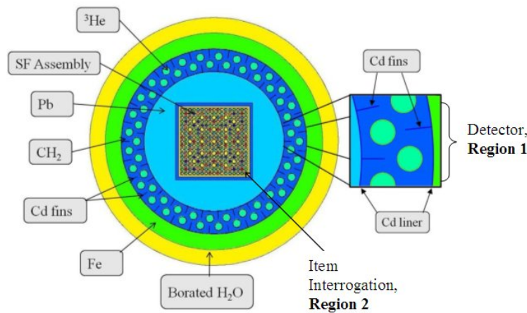
Figure 4: MCNPX design for PNA-R- 3 He detector hardware shown in the no Cd-liner configuration.
