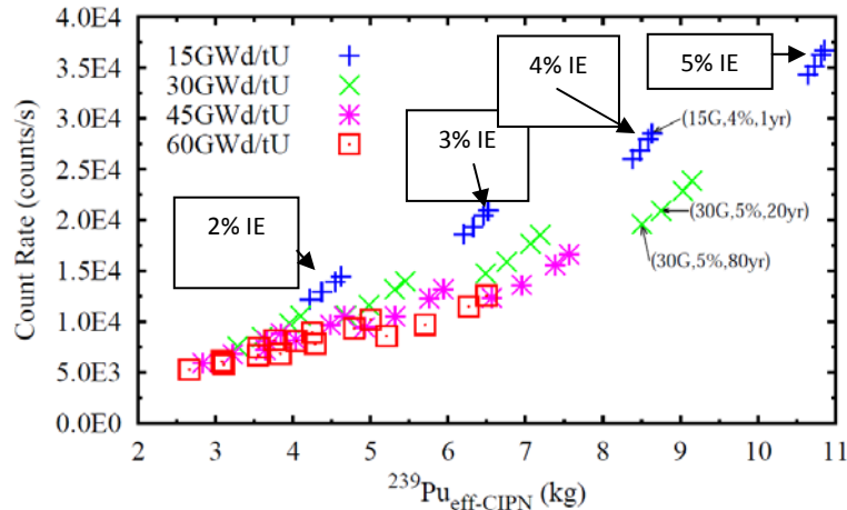
Figure 7: CIPN count rate vs. ^{239}\text{Pu}_{\text{eff-CIPN}} for the 64 assemblies in the spent fuel library for a ^{252}\text{Cf} source of 2 \times 10^8 n/s. The BU, IE and CT for 3 assemblies are individually labeled to give the CT structure.
