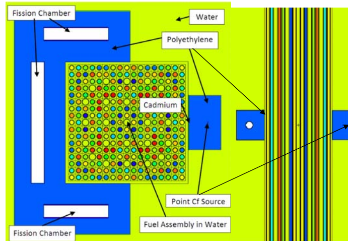
Figure 6: Plan and vertical cross sections of CIPN (not to scale).
