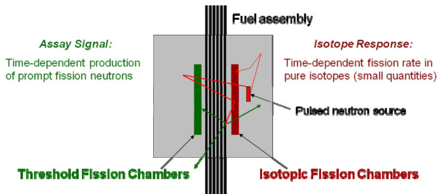
Figure 10: Schematic of a nominal lead-slowing-down spectrometer for spent nuclear fuel assay.
