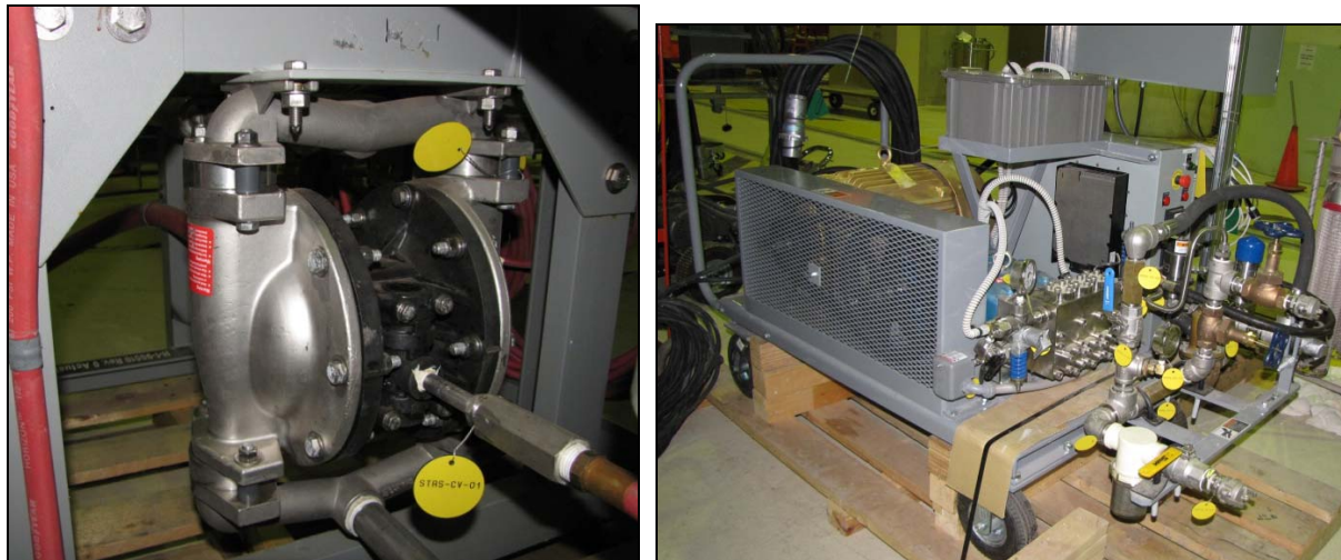
Figure 5. AODD Pump Mounted on Skid and High Pressure Pump Cart
