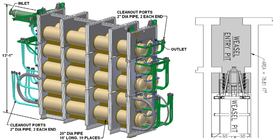
Figure 1. IWTS Settler Tanks
