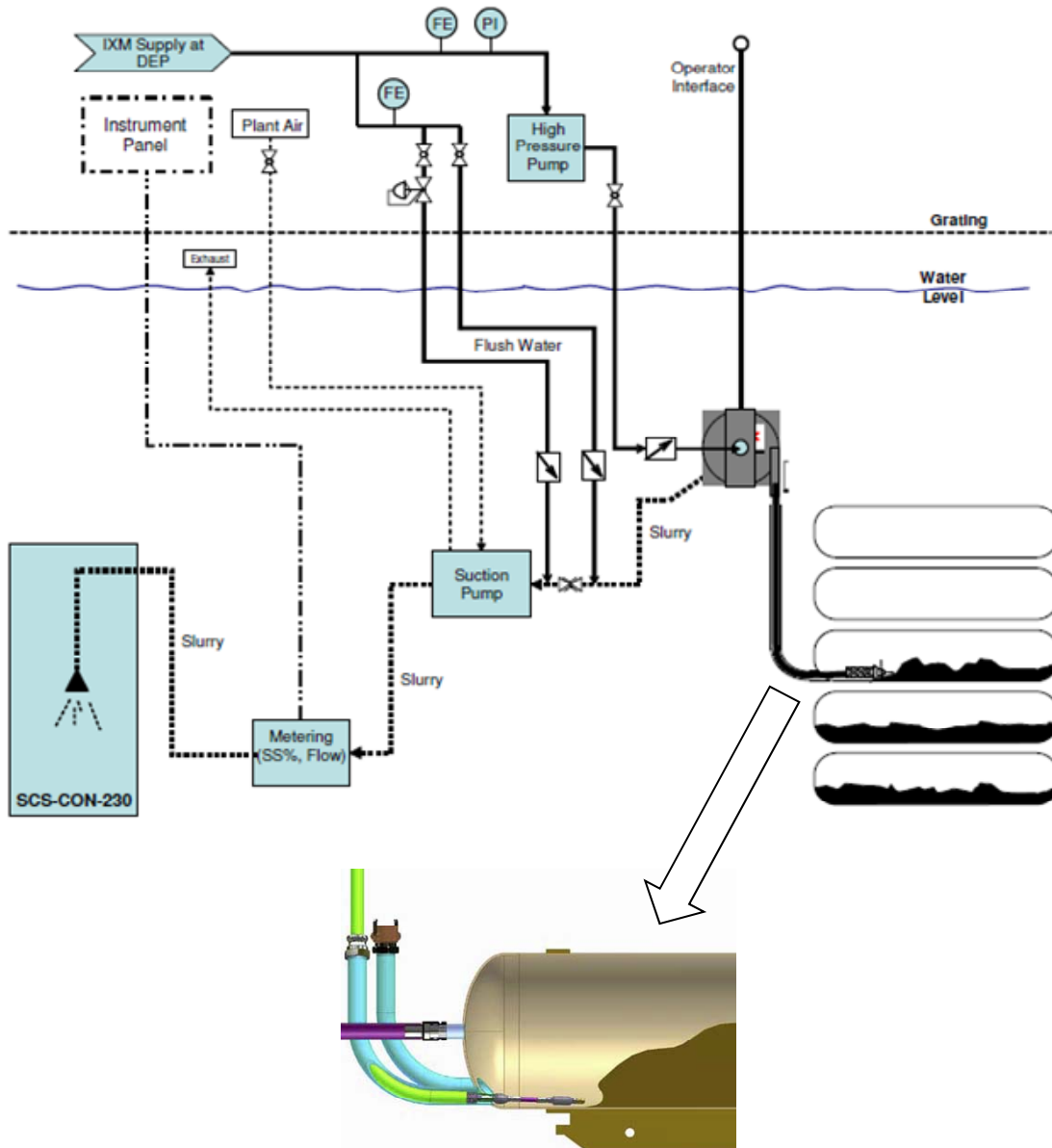
Figure 2. STRS Schematic and General Arrangement
