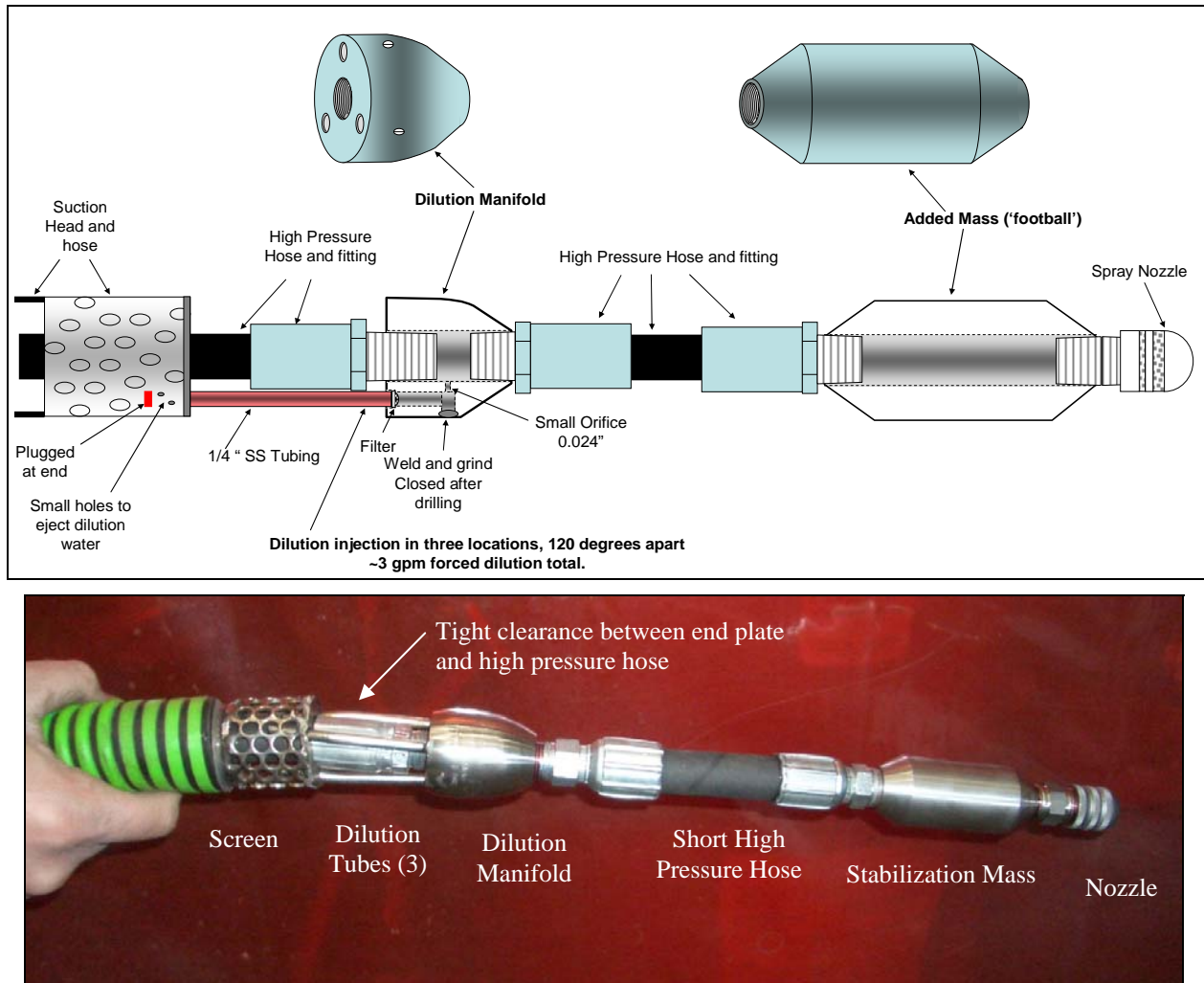
Figure 3. STRS Retrieval Head Design
