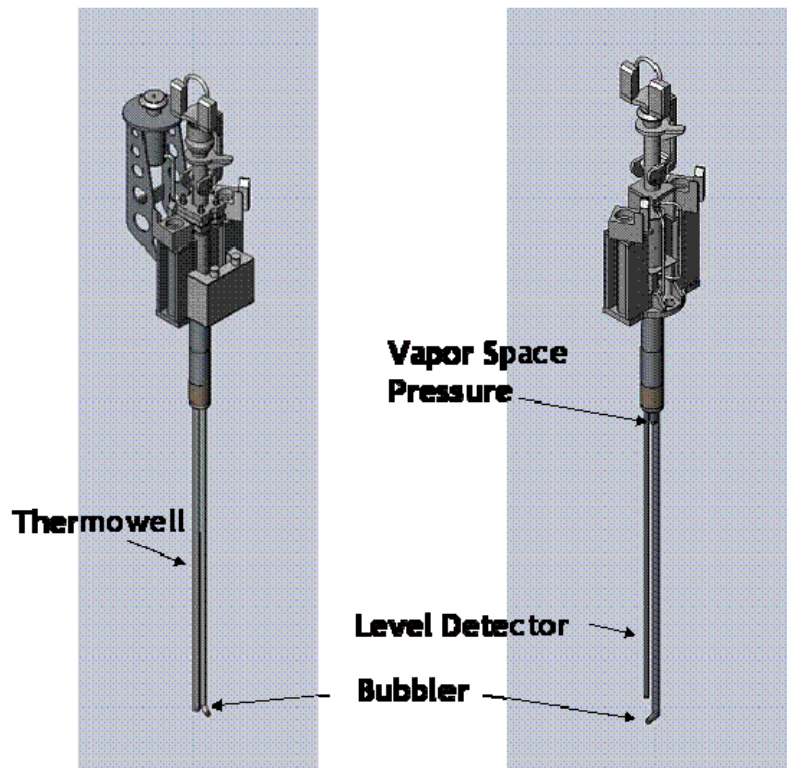
Fig. 3. Dual Function C4 Thermowell/Bubbler (Left) and C2 Level Probe/Bubbler (Right)
