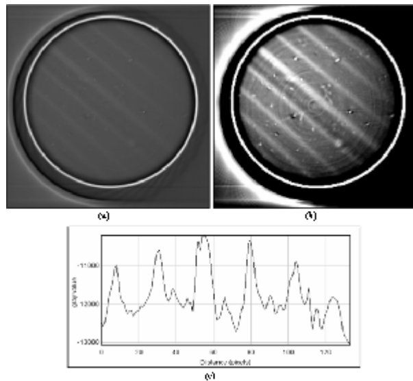
Figure 2: RadBall N-2-2 (a) Pre (b) Post Enhanced Contrast Optical CT Scan Images (c) Plot Profile.
