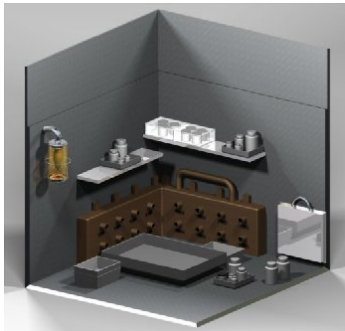
Figure 9: 3D Visualization of the Hot Cell in the SRNL Shielded Cells Facility.
