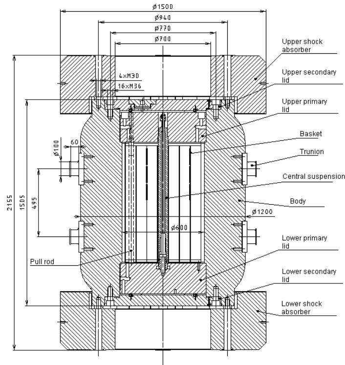
Fig. 3. Scheme of the VPVR/M cask.
