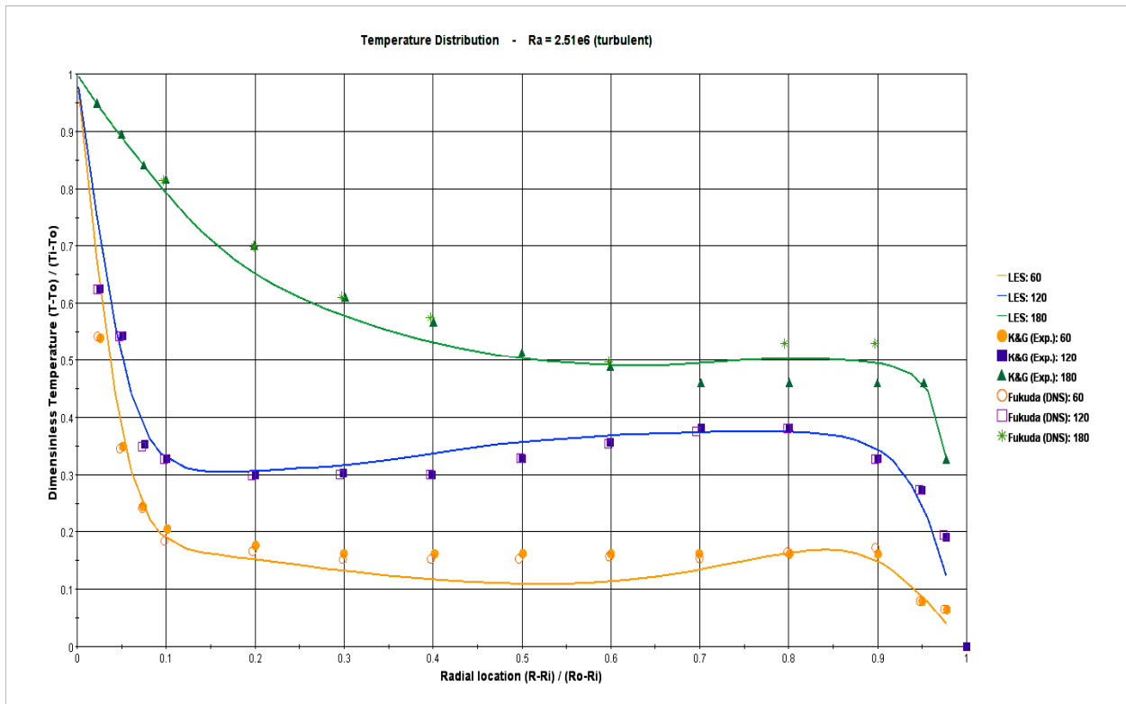
Figure 4: Temperature Profiles for LES ( Ra = 2.51 \times 10^6 ) with experimental data
