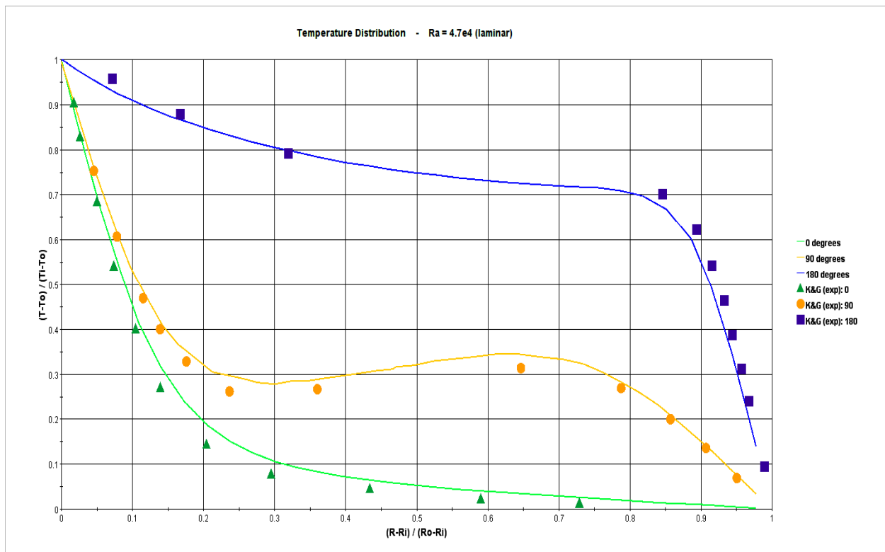
Figure 2: Laminar Temperatures Profiles ( Ra = 4.7 \times 10^4 ) for the two-dimensional, 1/2 symmetry model and Kuehn & Goldstein experimental data. Note: Angles are measured from the bottom ( 0^\circ ) to the top ( 180^\circ ) in all figures.
