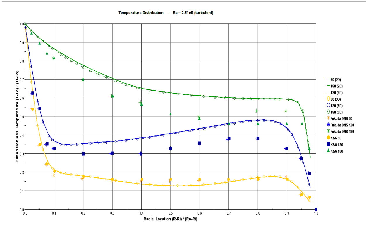
Figure 3: Temperature Profiles for RANS with steady and symmetry assumptions ( Ra = 2.51 \times 10^6 ) with experimental data. 2D and 3D data is also compared.
