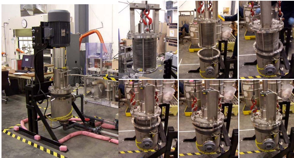
Fig. 1 Rotary filter system installed and insertion of disk stack into filter housing
