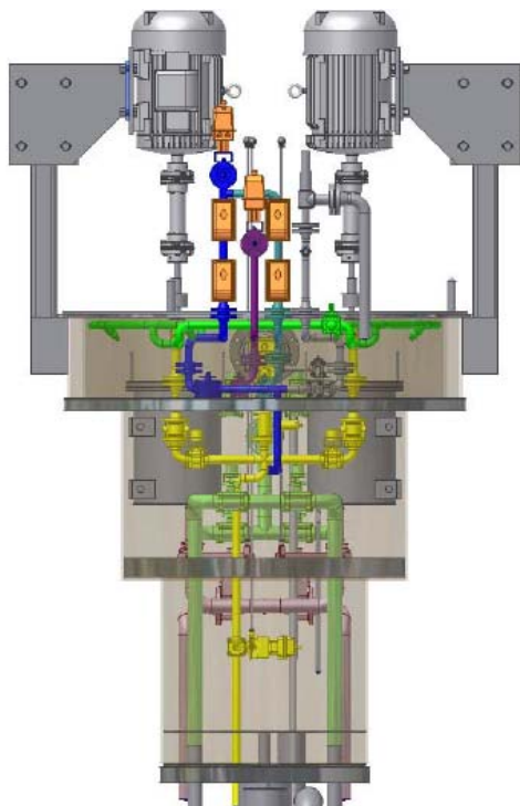
Fig. 4. Conceptual drawing of the plug portion of the EPRR pump/filter module
