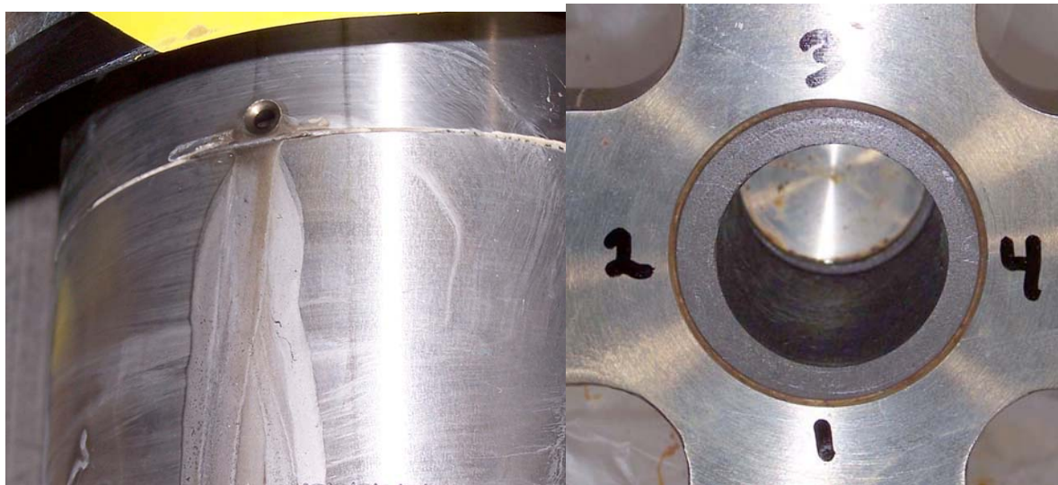
Fig. 8 Traces of filtrate drips from rotary joint upper weep hole (left) and wear on graphite bushing due to misalignment (right)
