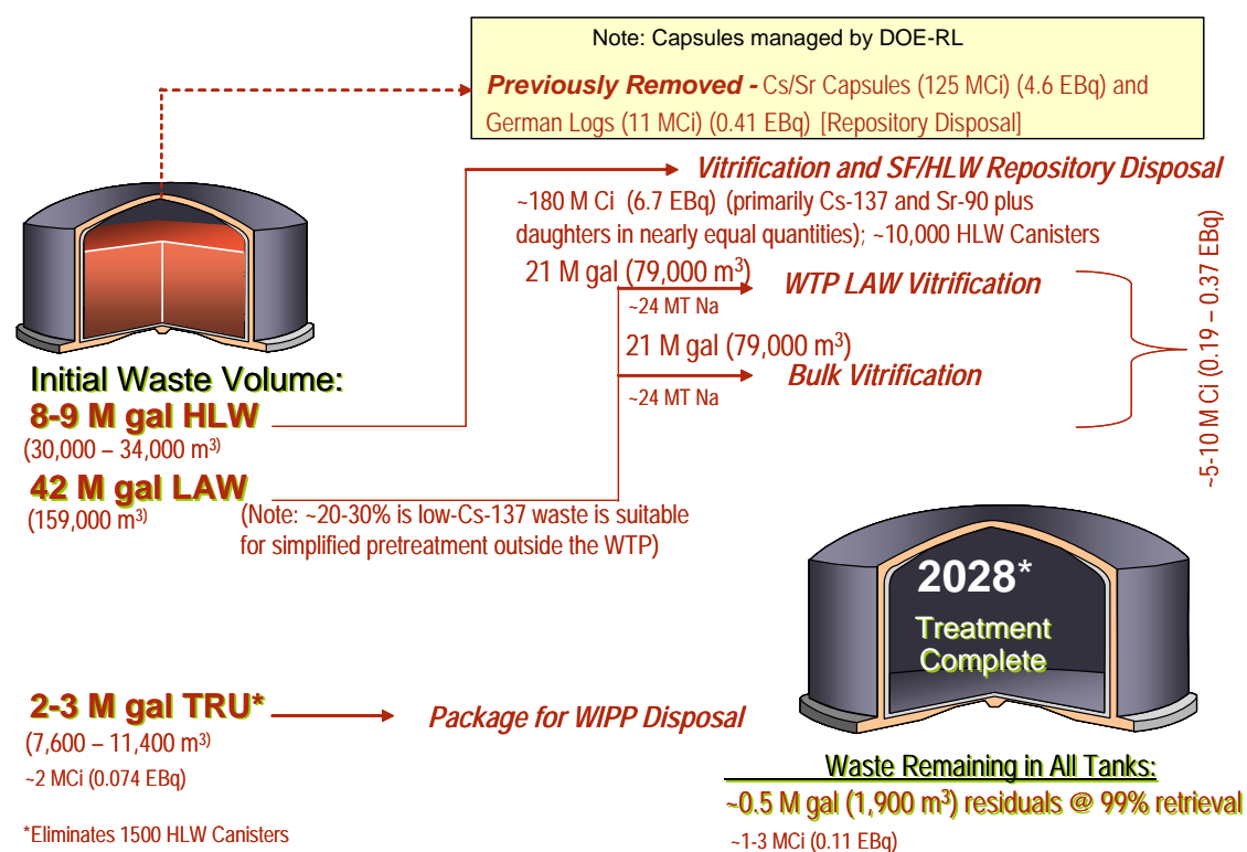
Fig. 1. General treatment and disposition scheme for Hanford tank wastes
