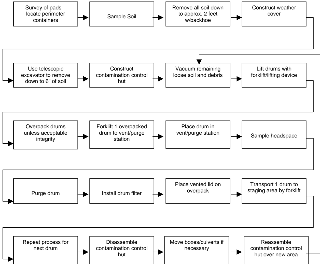
Fig. 2. Initial process envisaged for remediation of TRU pads
