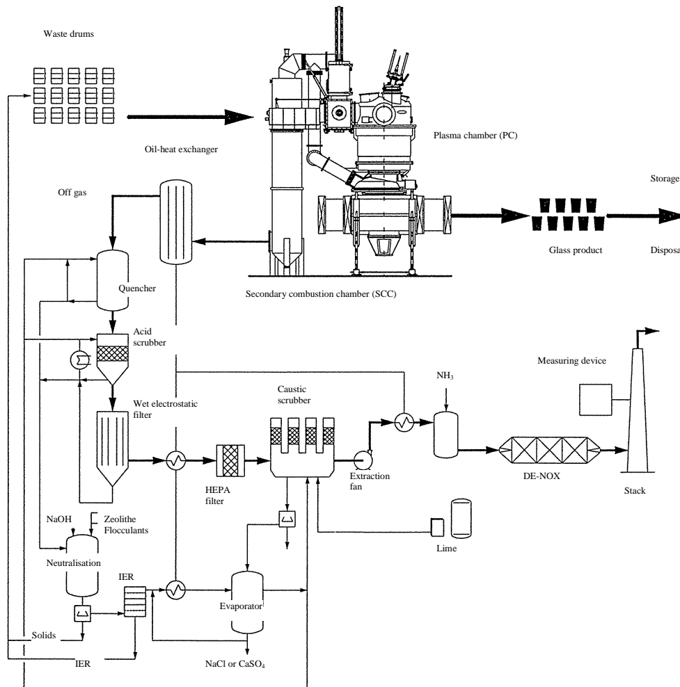
Fig. 6. ZWILAG PACT™ System flow sheet 7
