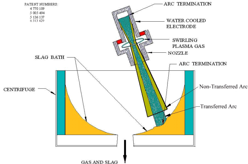
Fig. 4. Dual mode plasma torch operation[4]
