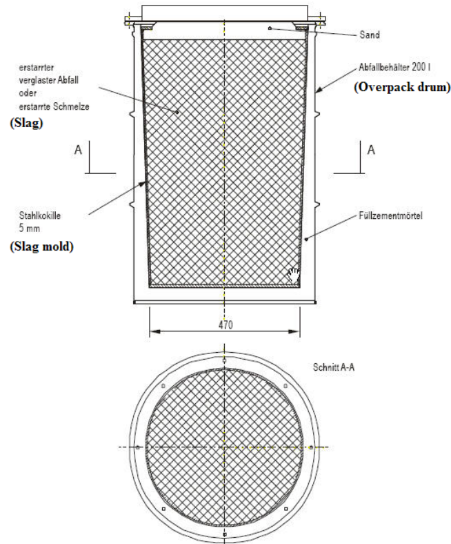
Fig. 7. Final storage mold and over pack drum
