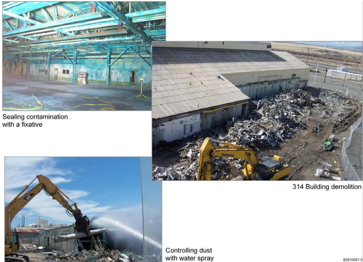
Fig. 2. Eliminating the spread of contamination during facility demolition
