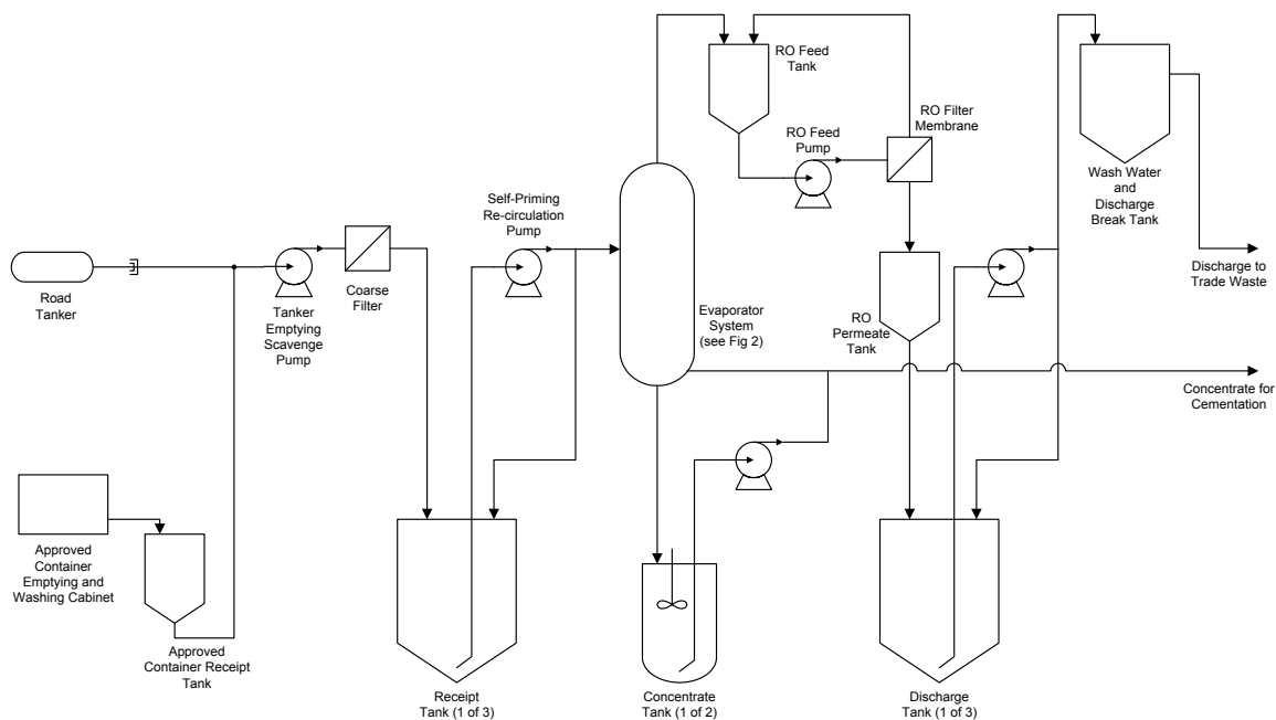
Fig 1. Overview of the WTP Process
