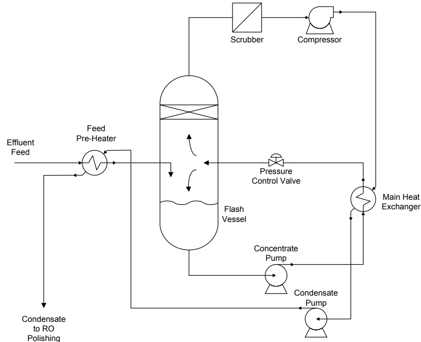
Fig 2. Evaporator MVR Circuit
