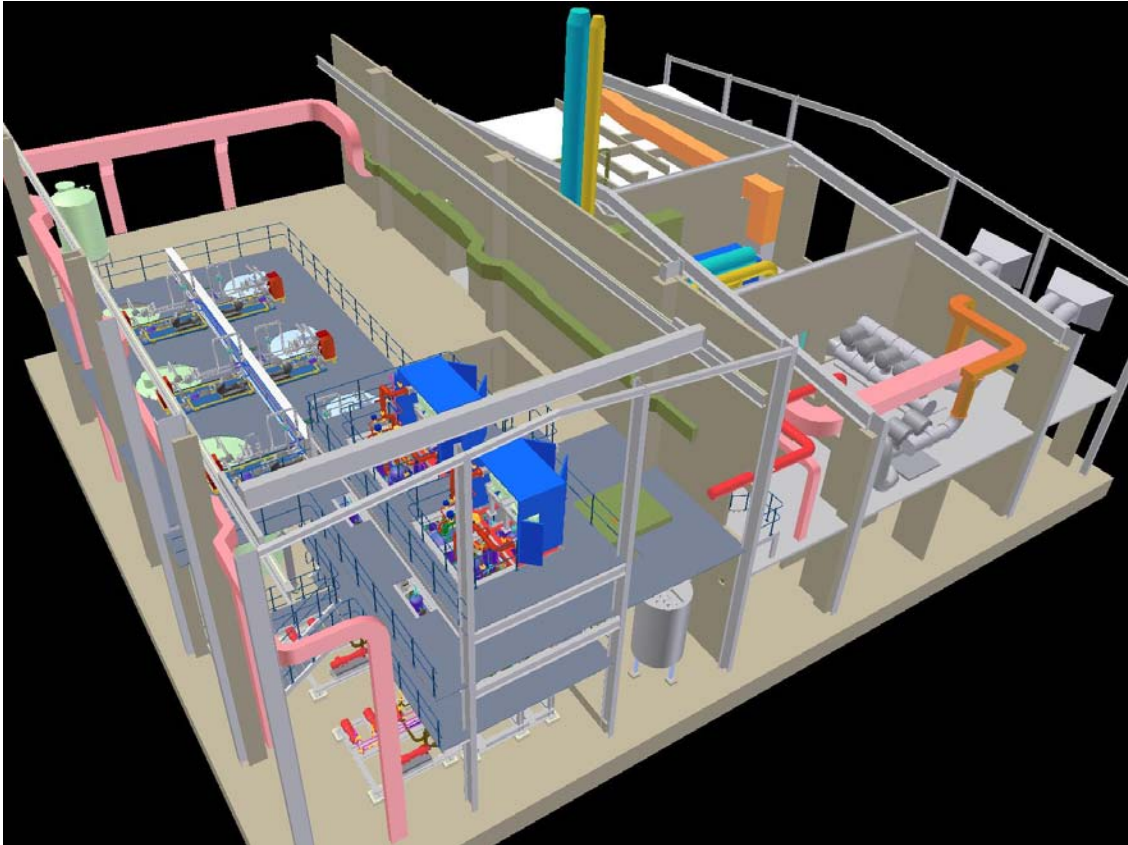
Fig. 3 3-D model picture of the WTP
