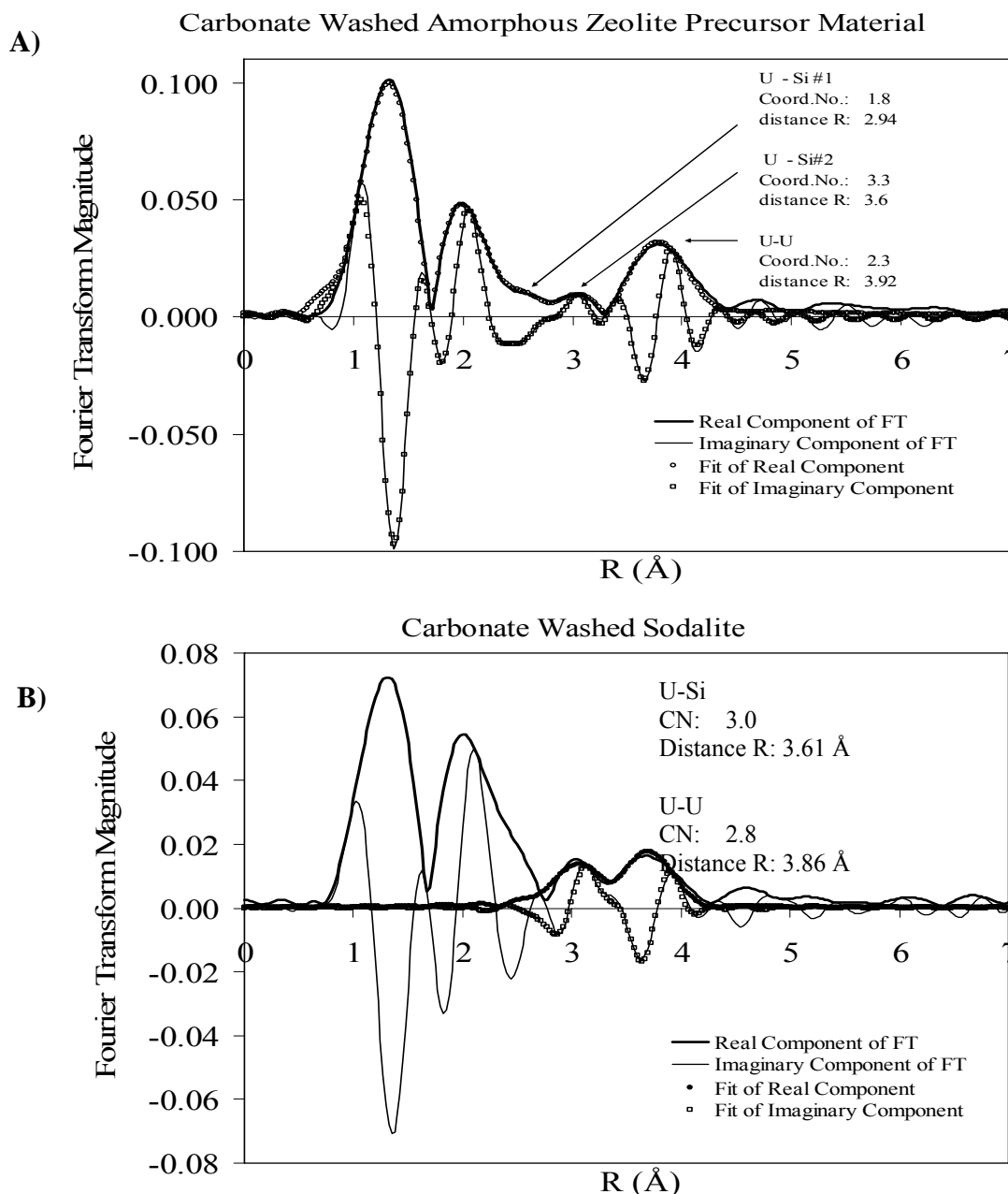
Fig. 4 Model fits for the outer shell components of the FT data for (A) carbonate-washed amorphous zeolite precursor and (B) carbonate-washed sodalite.
