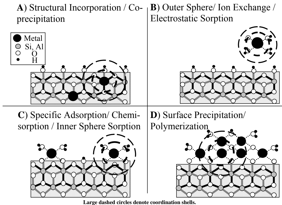
Fig. 1 Simplified diagram of the types of associations a metal could have with a surface: A) Structural incorporation/co-precipitation, B) Outer-sphere (electrostatic) sorption, C) Specific or inner-sphere sorption and D) Surface precipitation. Dashed rings denote first, second and third shell environments that can be probed with X-ray absorption fine-structure (XAFS) spectroscopic techniques.
