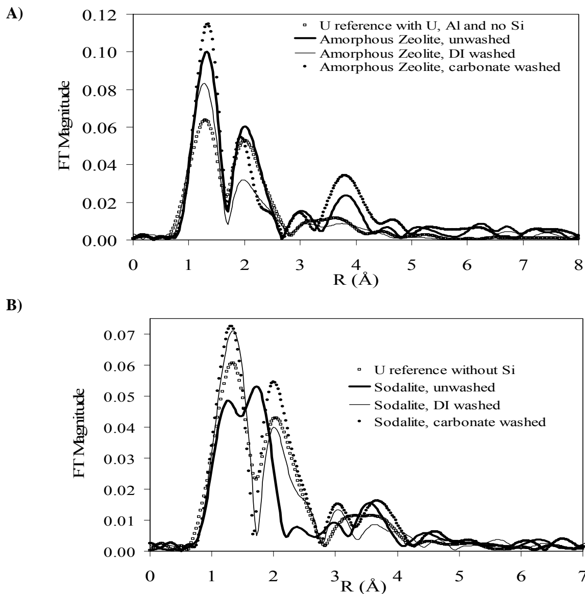
Fig. 3 FT data for the (A) amorphous zeolite and (B) sodalite series samples—uncorrected for phase shift.
