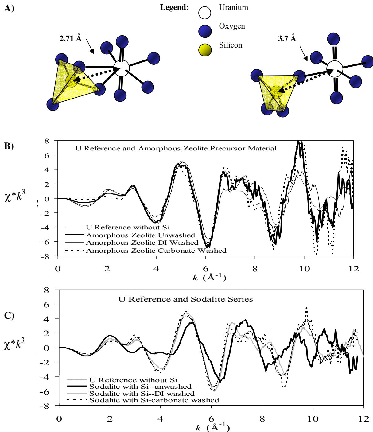
Figure 2 (A, left) In published U-XAFS literature on uranyl sorption to silica gels, the U-Si distance of \sim 2.71 \text{\AA} (dashed arrow) and has been interpreted as edge-sharing. Hence, short U-Si distances without long radial distances are a typical signature for sorption. In published U-EXAFS literature for uranyl silicates, the U-Si distance is \sim 3.7 \text{\AA} (dashed arrow, A, right ), which is indicative of corner-sharing. Long U-Si distances typically signify structural incorporation of U (i.e., longer radial distances are needed for a lattice environment as opposed to a sorption-type environment). (B) and (C) represent chi data for the amorphous zeolite and sodalite series (respectively).
