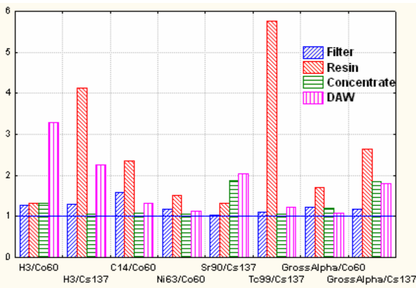
Fig. 2 The ratios of arithmetic mean and geometric mean for each waste type and pairs of radionuclides
