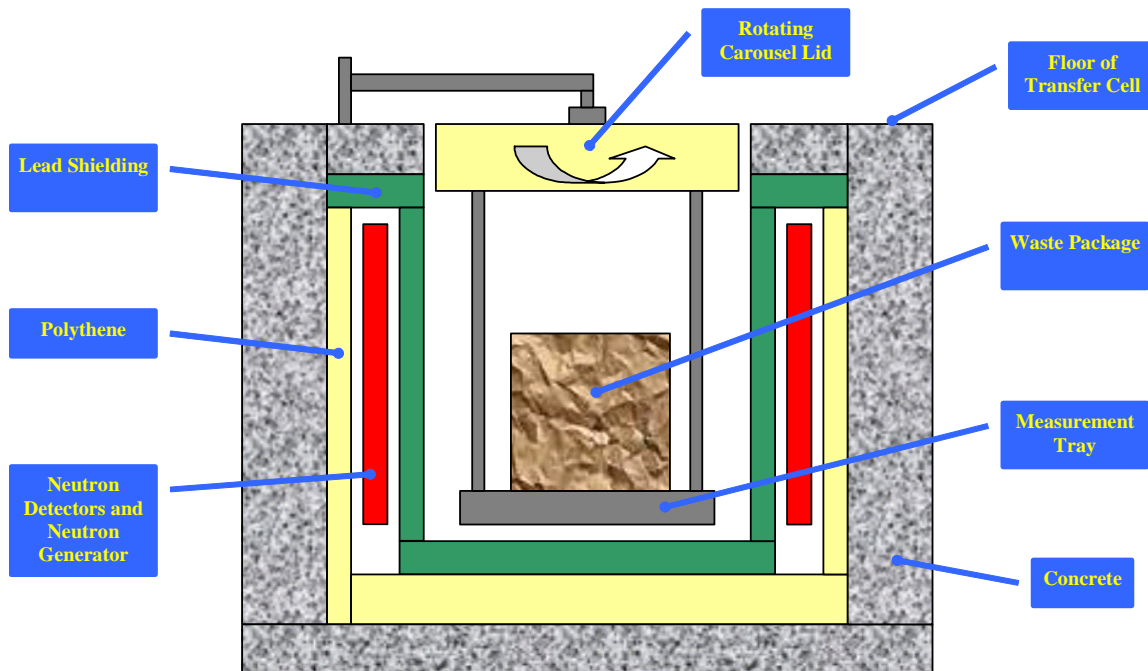
Fig. 2 Schematic of Fissile Material Detector
