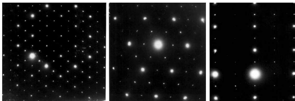
Figure 4. SAED patterns of the pyrochlore structure phase from the planes of inverse lattice [(110)* – left, (111)* – middle, (211)* - right] in the samples M24 (left and middle) and A/3/6 (right).
