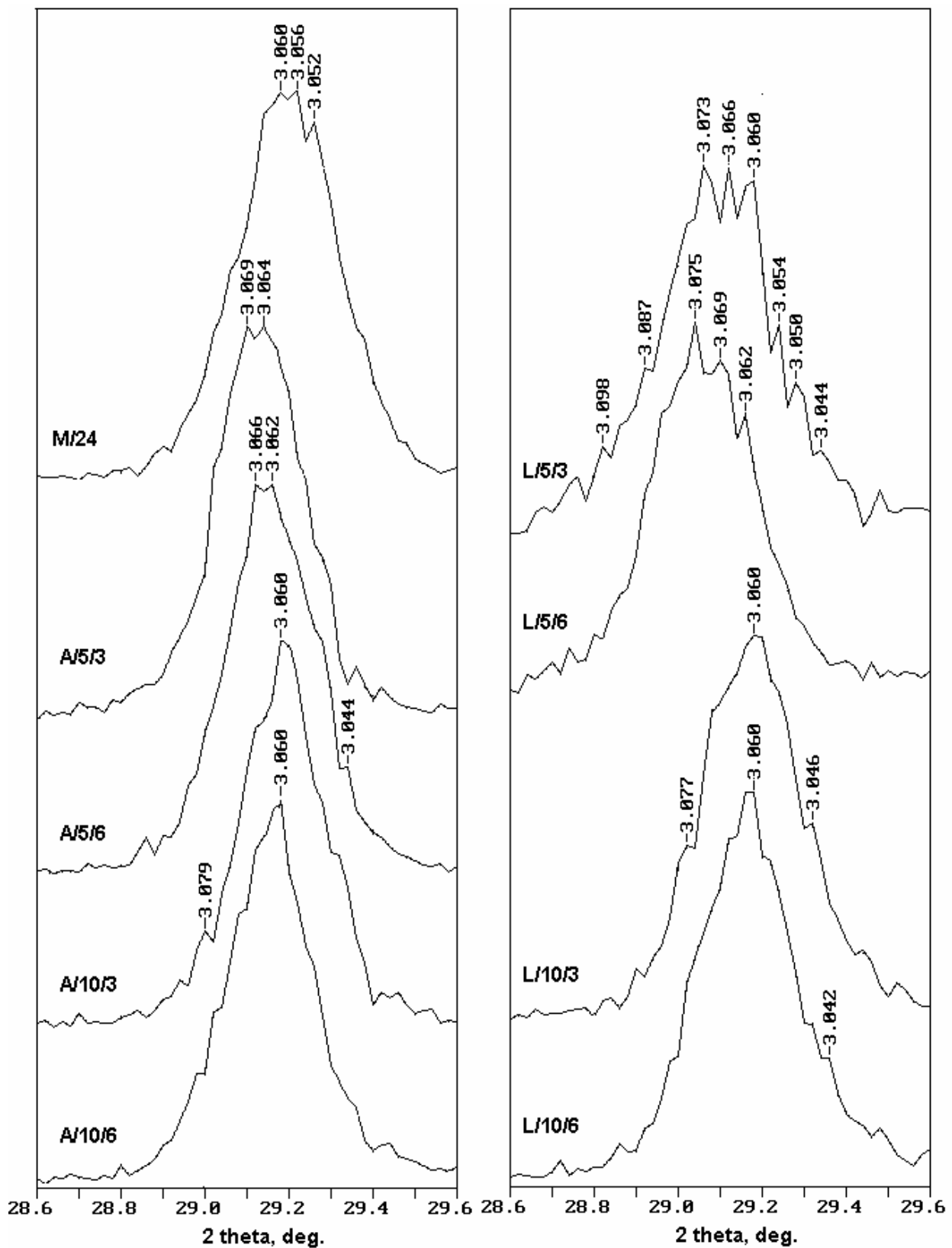
Figure 2. Splitting of the major pyrochlore reflection (222) on XRD patterns of the ceramic samples.
