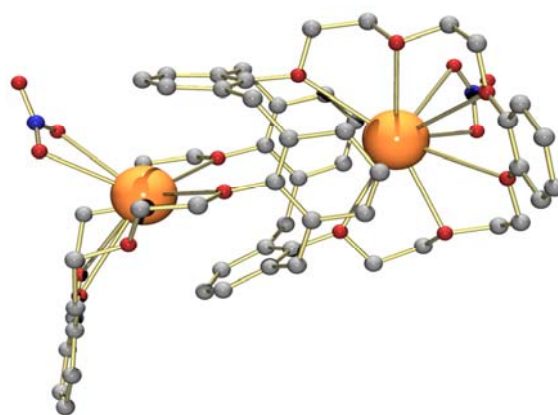
Calix[4]arene-bis(8-octylbenzo-crown-6) "BOBCalixC6" (As complexed with Cs + ion)
