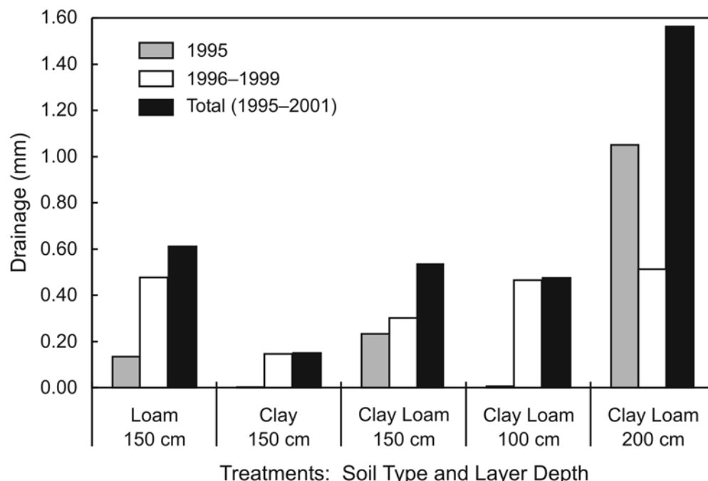
Figure 3. Small lysimeter drainage values for all treatment combinations for 1995, 1996–1999, and the total for 1995–2001. Drainage values for 2000 and 2001 are insignificant and are not displayed.
