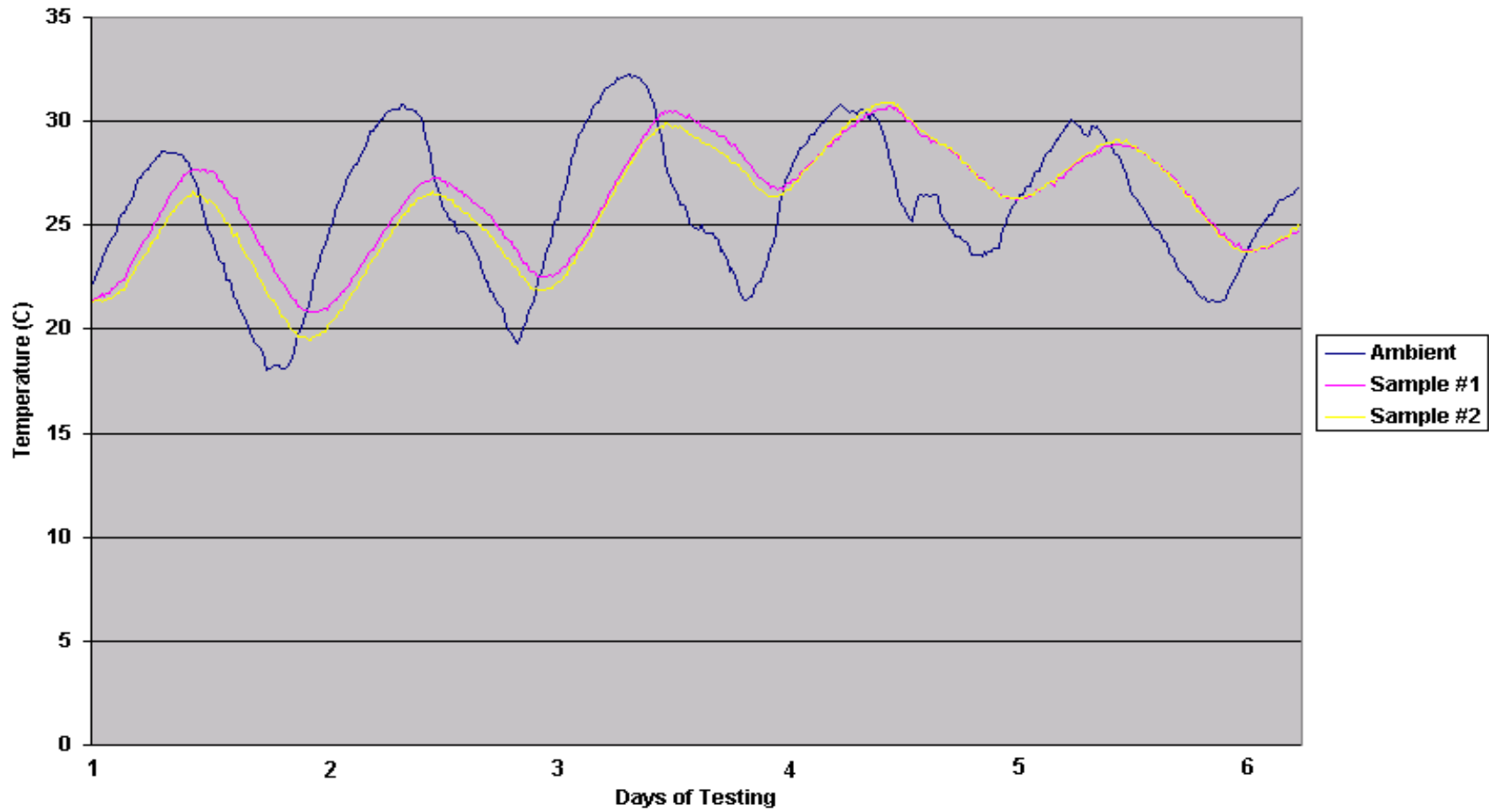
Fig. 2. Heat Release Test of Grout Mixture with 603 Basins Water Concentrate (#2)
