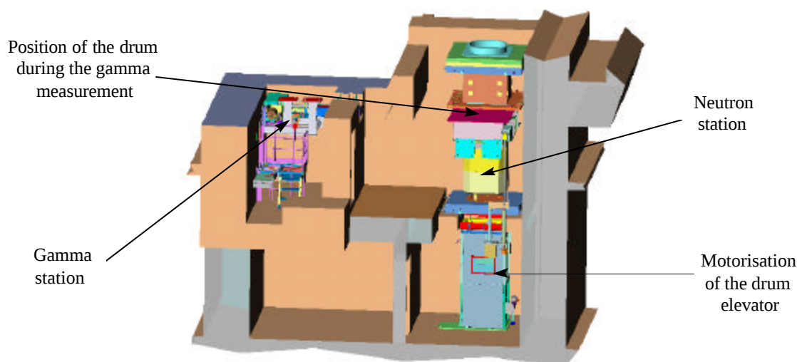
Fig. 1. General layout of the incoming measurement station
