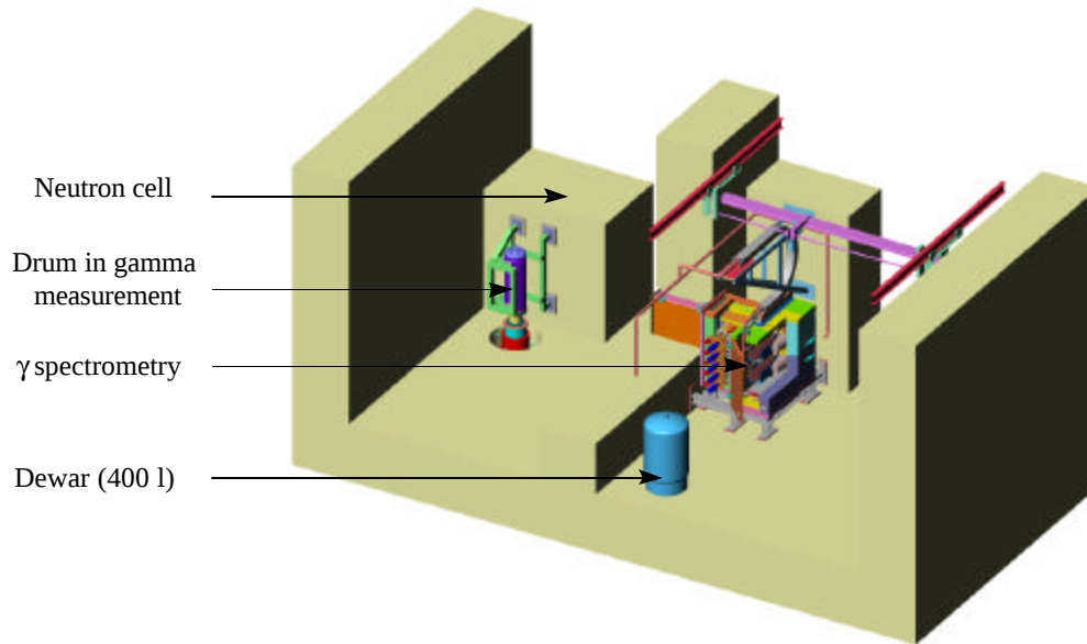
Fig. 4. General layout of the measurement station
