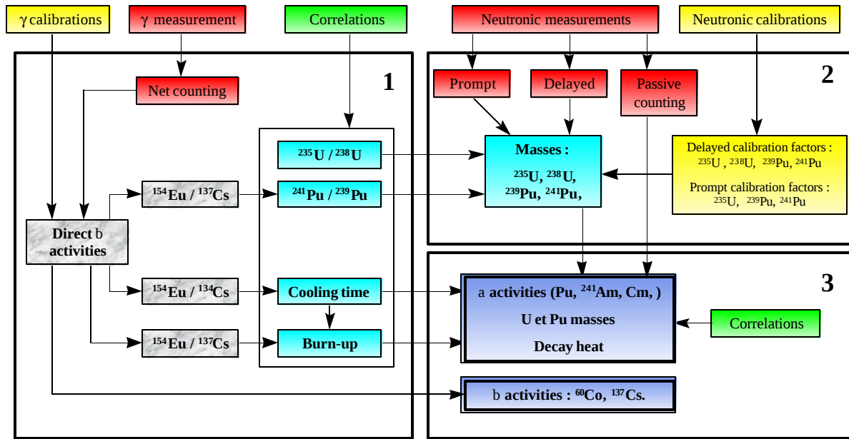
Fig. 9. Three measurement interpretation phases
