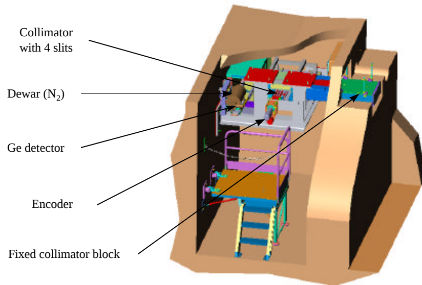
Fig. 2. Details of the Gamma Spectrometry Station Layout
