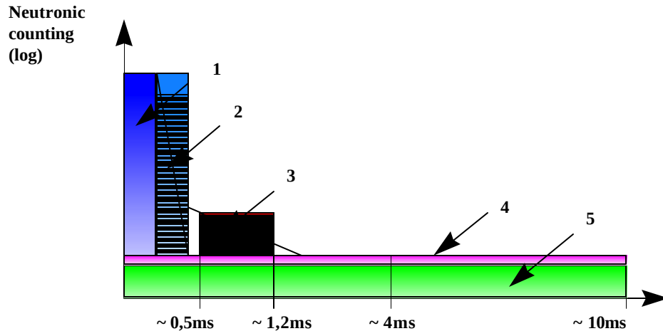
Fig. 8. Measurement cycles
