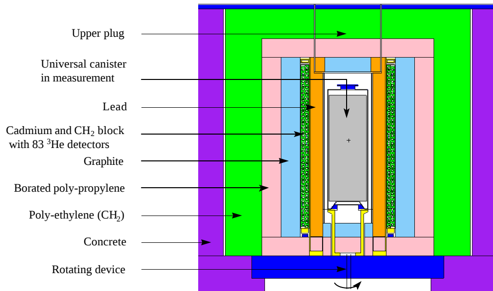
Fig. 5. Vertical view of the measurement station
