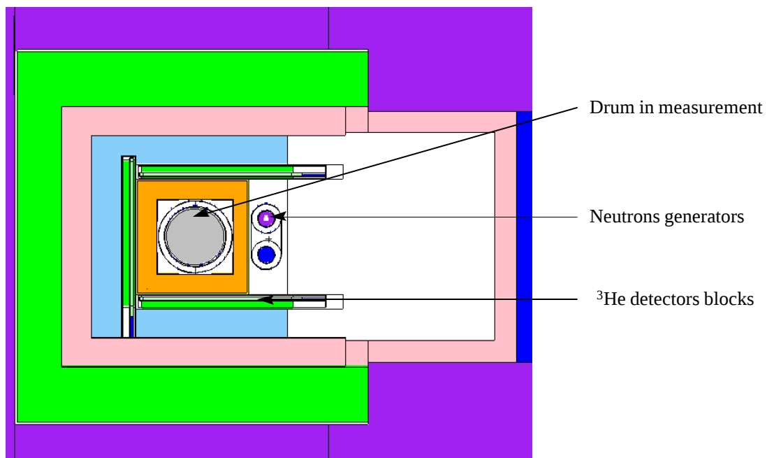
Fig. 6. Horizontal view of the measurement station
