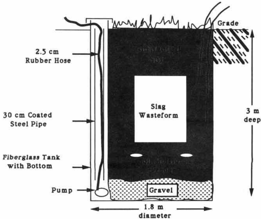
Fig. 1B. Schematic diagram of the lysimeter apparatus containing the slag formulation monolith of saltstone.
