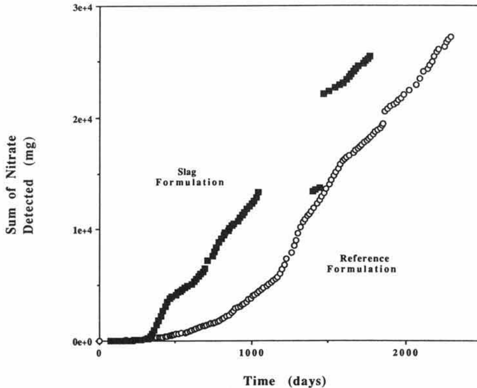
Fig. 2A. Total nitrate (mg) detected in the sumps of the lysimeters with time.
