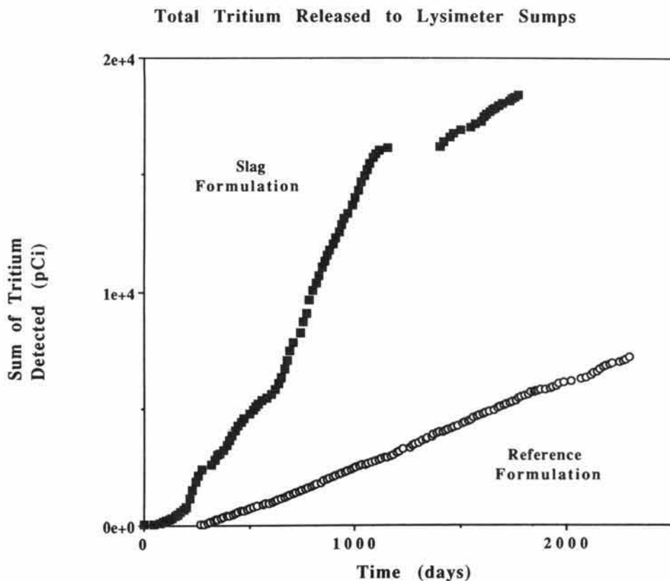
Fig. 2B. Total tritium (pCi) detected in the sumps of the lysimeters with time.
