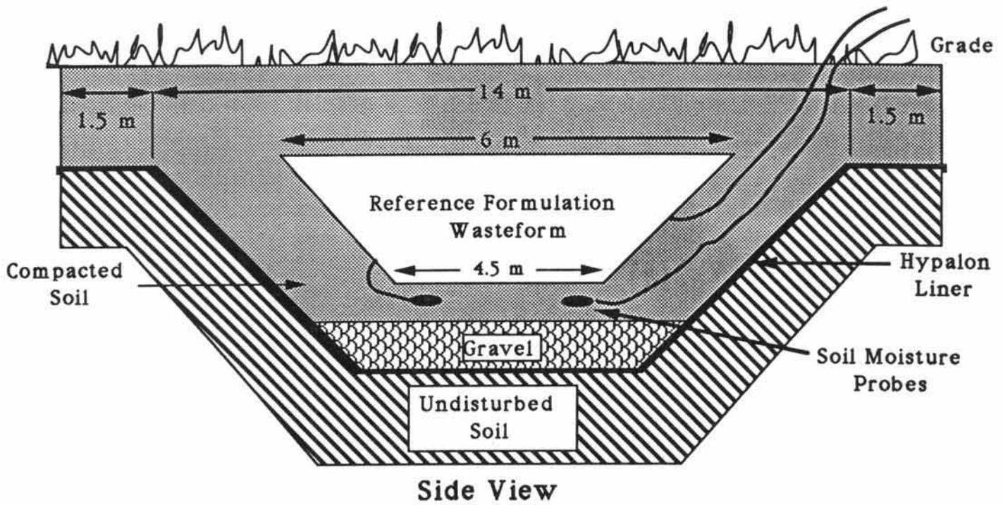
Fig. 1A. Schematic diagram of the lysimeter apparatus containing the reference formulation monolith of saltstone.
