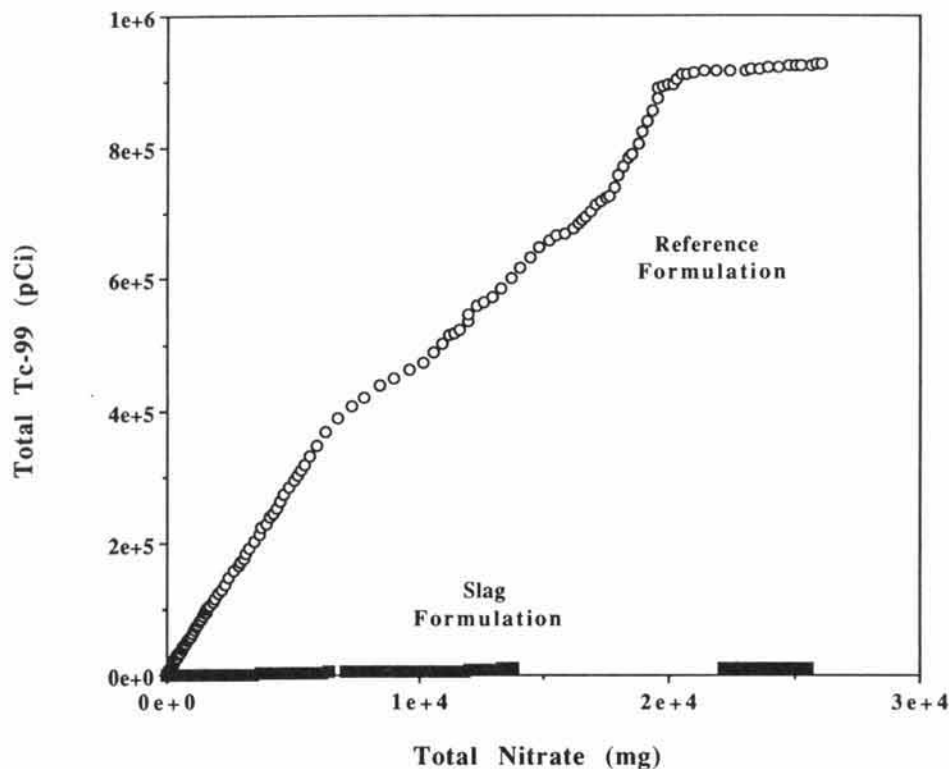
Fig. 3. Total technetium-99 detected plotted as a function of the total nitrate detected in the sumps.
