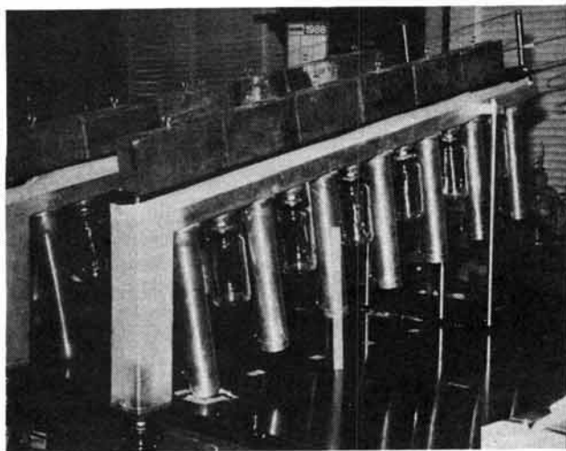
Fig. 20. Mini-soil beam used for evaluation of materials for possible use in conductive layer barrier application. This soil beam has a total length of 4.5 ft.
