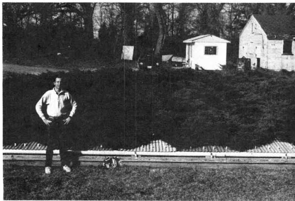
Fig. 5. Bioengineering plots at Beltsville. Photo taken in January of 1991, four years after planting of Pfitzer junipers. Run-off is 70% of precipitation.
