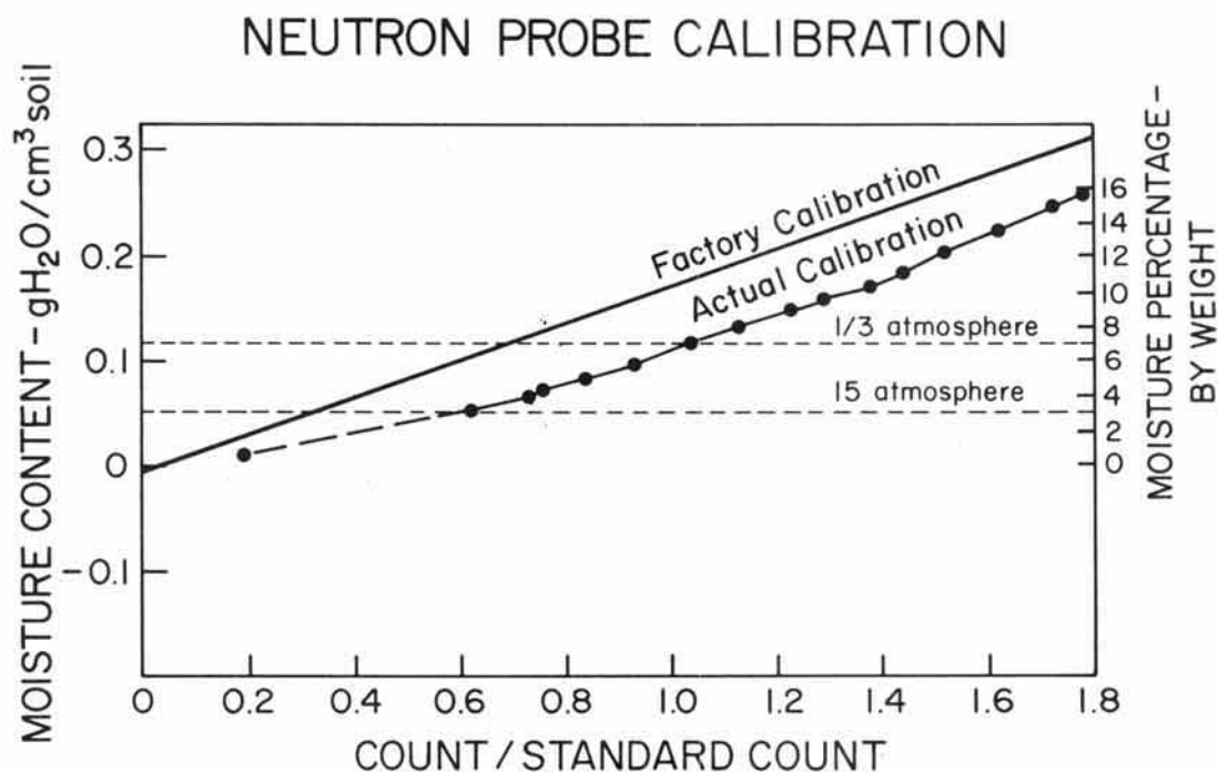
Fig. 10. Calibration of neutron probe using soil of bioengineered lysimeters. Calibration was carried out in a weighing lysimeter over a three-year period. Factory calibration was supplied by manufacturer of neutron probe and was made against sand rather than soil.
