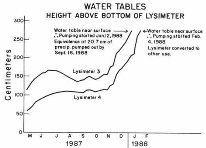
Fig. 7. Water table vs. time in reference lysimeters. The crowned surface is cropped with fescue grass. Water table increased with time until pumping of water table was necessary to keep trench from running over. Surface run-off was 8% of precipitation.
