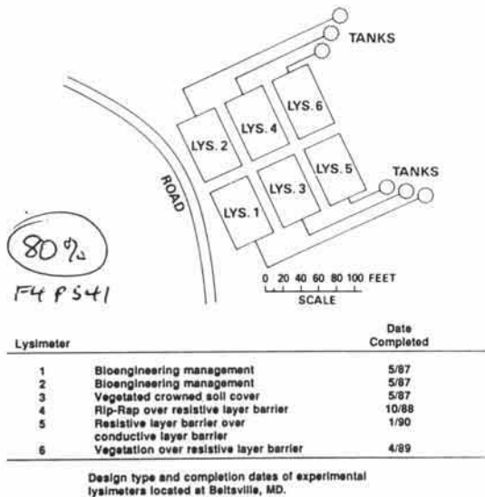
Fig. 4. Plan view showing placement of experimental lysimeters at Beltsville, MD.
