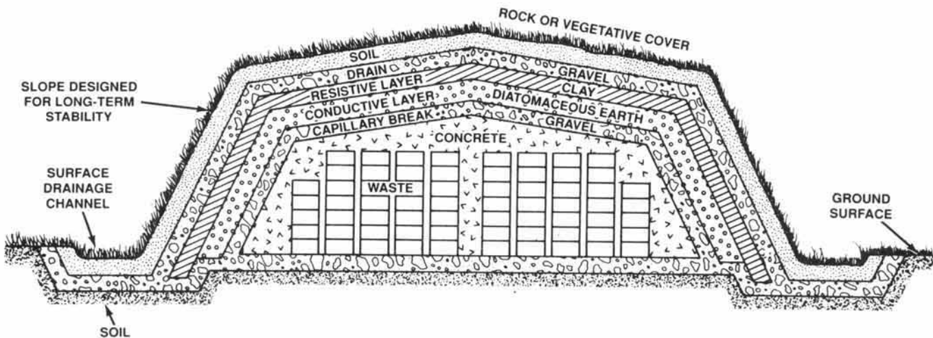
Fig. 25. Resistive layer barrier overlaying a conductive layer barrier as it might be used with an earth-mounded concrete bunker. The resistive (clay) layer is the primary barrier to water passage downward. The conductive layer (diatomaceous earth) will scavenge and conduct any water leakage around the concrete structure to drains. The diatomaceous/gravel interface is the capillary break. The concrete is exposed only to a stagnant, alkaline film of water which will greatly retard the degradation of the concrete over a very long time period. Only geological materials already over one million years old are used in construction, other than the concrete, so the life of the cover will far exceed that of the concrete, even though this cover system can be expected to significantly increase the structural life of the concrete.
