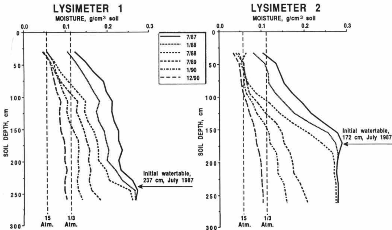
Fig. 11. Bioengineered covers. Volumetric soil moisture content plotted as a function of soil depth at six different dates. By July of 1989 water table had been eliminated from soil profiles. By December of 1990 entire soil profiles, although relatively dry, still showed increasing moisture content with depth.
