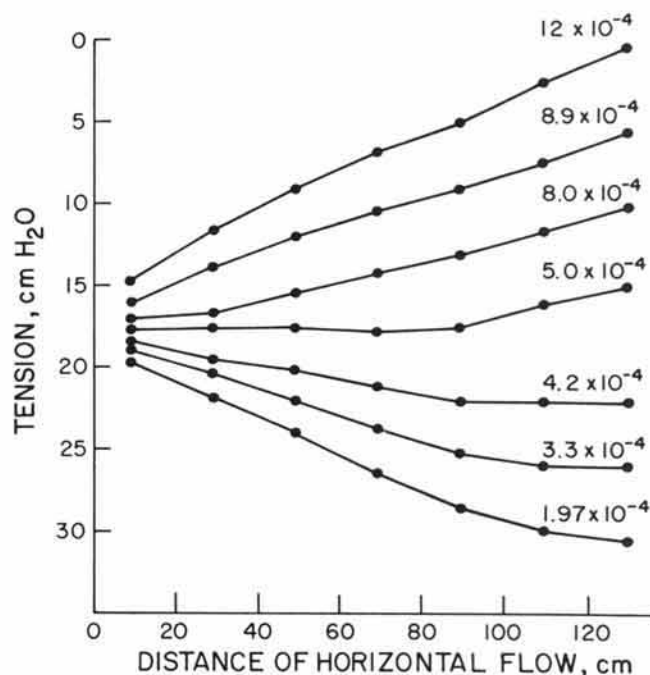
Fig. 21. Soil water tension at various flow rates. Tension vs. horizontal distance from discharge point. Results suggest that at rates of 4.2 \times 10^{-4} cm/sec or less, water would remain under tension at any beam length.
