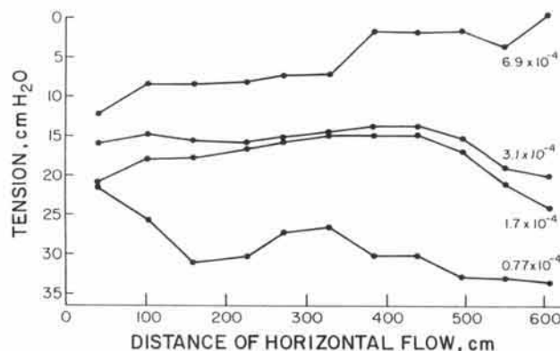
Fig. 23. Soil water tension at various flow rates and as determined over a 21 ft long flow distance. At -15 to -20 cm, matric potential water flow rate is approximately 3 \times 10^{-4} cm/sec. At this flow rate unsaturated flow can be maintained over an infinite distance which confirms the results of the mini-beam measurements (Fig. 21).
